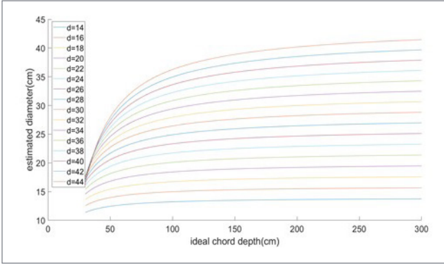
Figure 1. Examples of estimated diameter function with different capture distances and tree sizes. In fact, for large capture distance the estimated diameter function is approximately linear and monotone on both tree size and capture distance.
