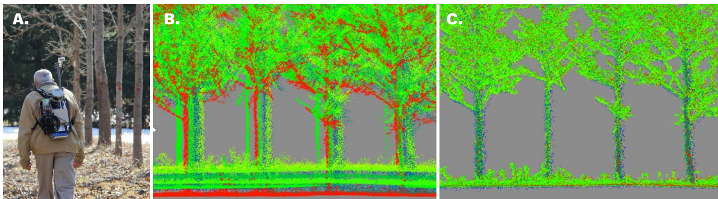
Figure 2. Backpack deployment in Martell Forest (a), and LiDAR point clouds before (b) and after (c) trajectory enhancement.
