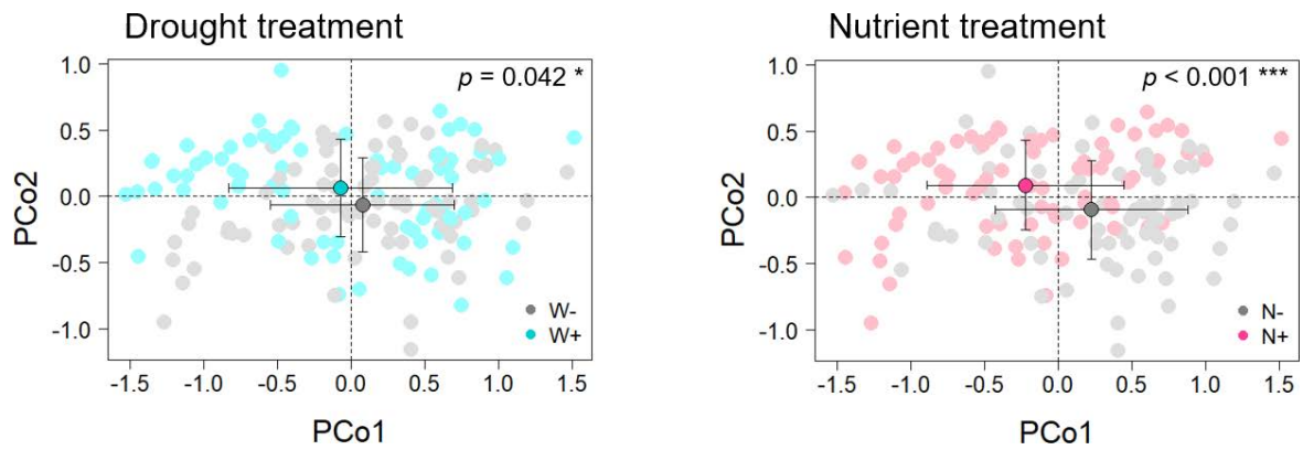
Figure 4. Scores (mean \pm standard error) for the first and second components from principal coordinates analysis (PCoA) of reflectance data (400–2400 nm) collected from walnut leaves in 2018, showing the ability of spectral data to discriminate control (blue circle; W+) versus black walnut with drought stress (grey circle; W-) in the left panel and control (pink circle; N+) versus black walnut with nutrient deficiency stress (grey circle; N-) in the right panel. P-values from permutational analysis of variance for the effects of the drought and nutrient deficiency stress on full range (400–2400 nm) reflectance profiles of walnut leaves are shown in the top-right corners of panels.
