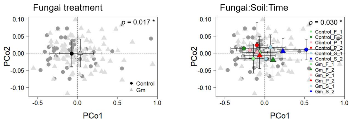
Figure 5. Scores (mean \pm standard error) for the first and second components from principal coordinates analysis (PCoA) of reflectance data (400–700 nm) collected from walnut leaves in 2018, showing the ability of spectral data to discriminate control (black circle; Control) versus black walnut inoculated with the fungus Geosmithia morbida (grey triangle; Gm) in the left panel and the interactions among fungal treatment (circle; Control vs. triangle; Gm), soil type (green; forest vs. red; plantation vs. blue; sterile soil) and time length after fungal infection (light; 1 vs. dark color; 2) in the right panel. P-values from permutational analysis of variance for the effects of the fungal infection, soil types, and time on reflectance profiles (400–700 nm) of walnut leaves are shown in the top-right corners of panels.
