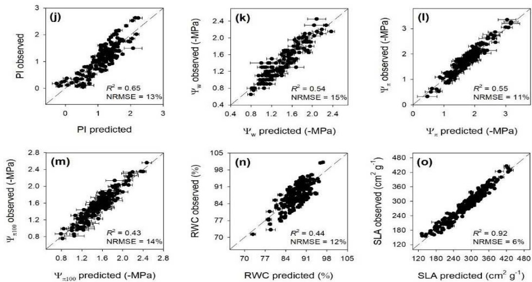
Figure 2. Observed vs. predicted values of leaf traits related with water status for black walnut and northern red oak exposed to various stressors. Error bars for predicted values represent the standard deviations generated from the 500 simulated models. The dashed line shows 1:1 relationship.
