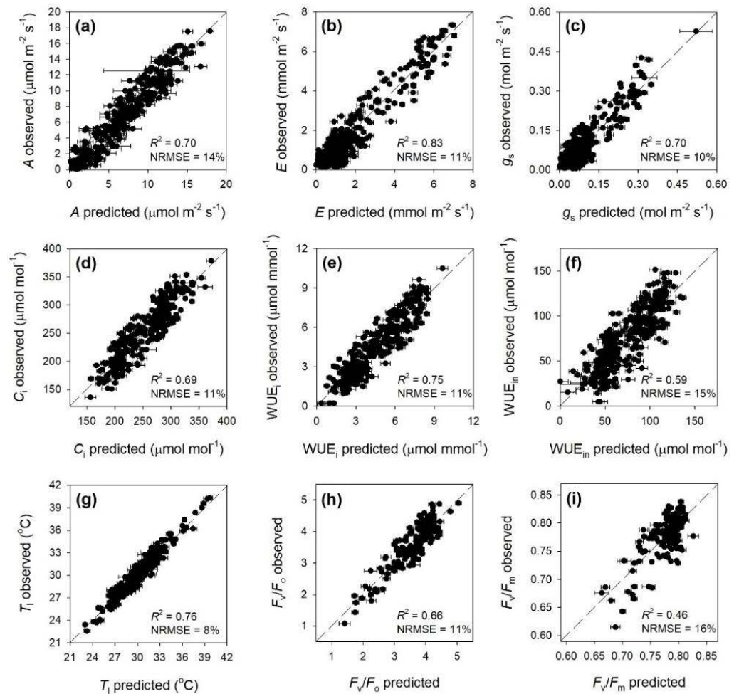
Figure 1. Observed vs. predicted values of leaf traits related with gas exchange parameters and chlorophyll fluorescence for black walnut and northern red oak exposed to various stressors. Error bars for predicted values represent the standard deviations generated from the 500 simulated models. The dashed line shows 1:1 relationship.
