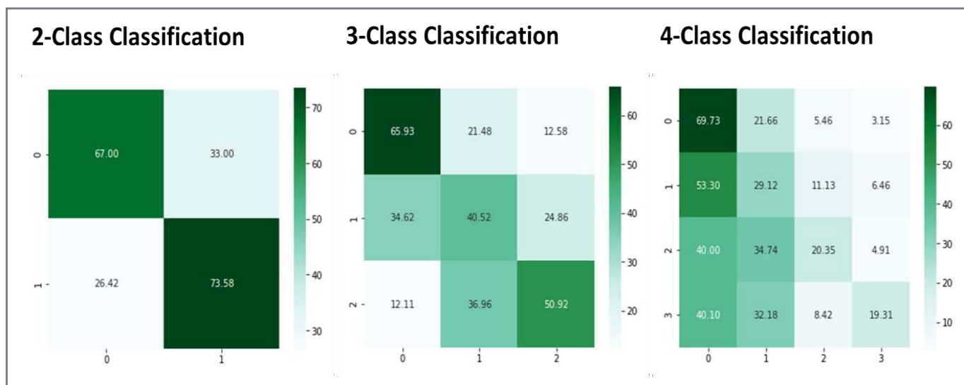
Figure 4. Confusion matrix based on classification. For example, in the far-left panel, a 0 (no blight) is accurately classified 67% of the time and misclassified as having blight 33% of the time. Notice that as classes are added more classes are confused.
