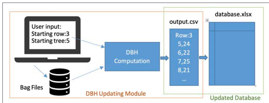
Figure 4. Illustration of automated tree ID patching and database updating.
