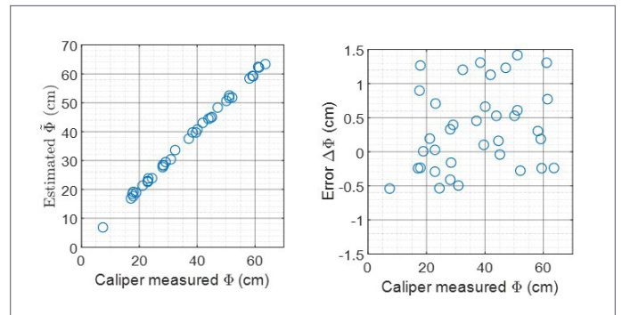
Figure 4. The behaviors of diameter estimation results and diameter error. The error is not notably influenced by capture distance.
