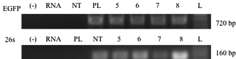
Fig. 5 RT-PCR analysis of pumpkin ash (PA) first-strand cDNA from transgenic and control non-transgenic leaves. Primers were used to specifically amplify the 720 bp EGFP and the 160 bp 26S.
